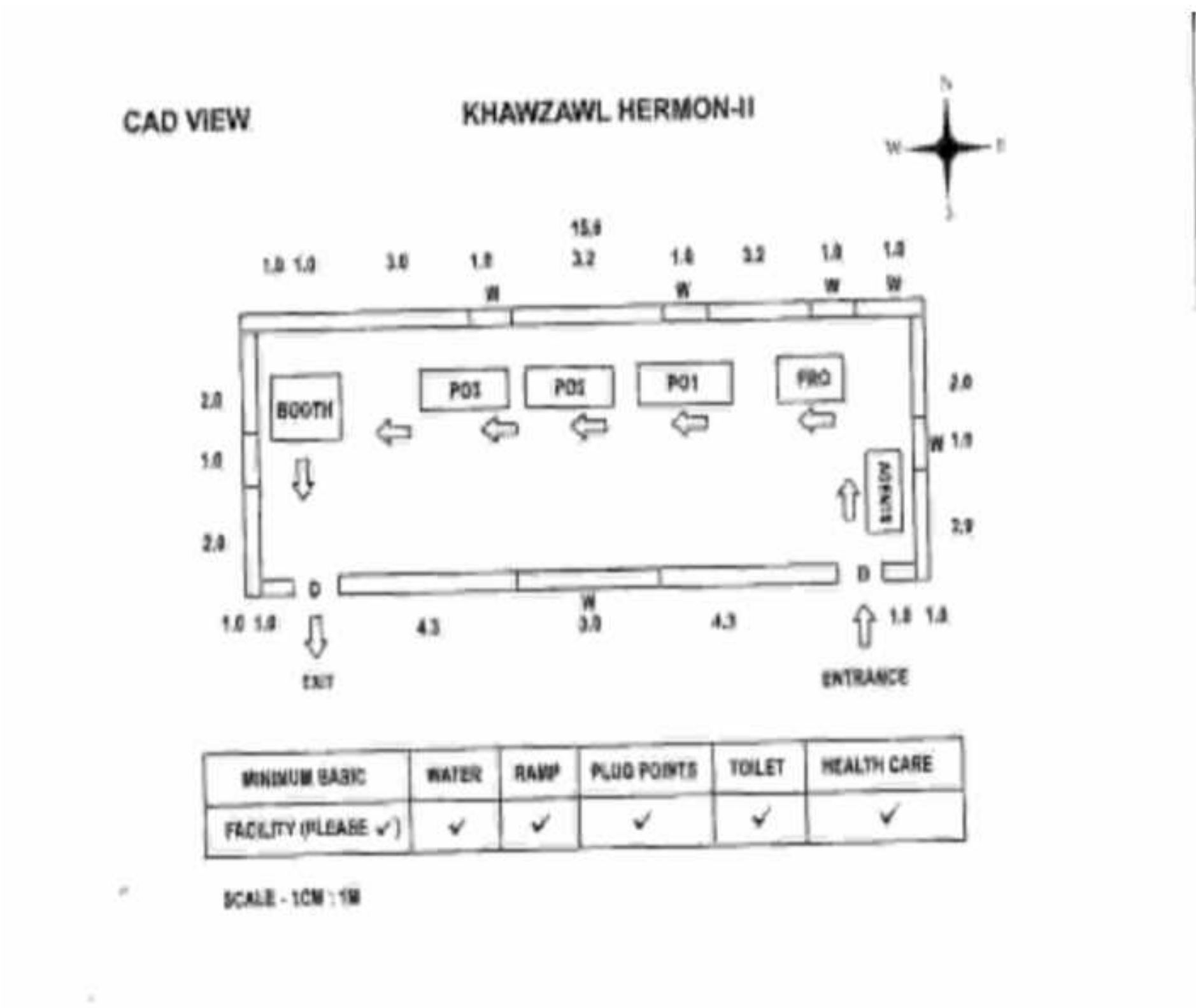
Cad View
