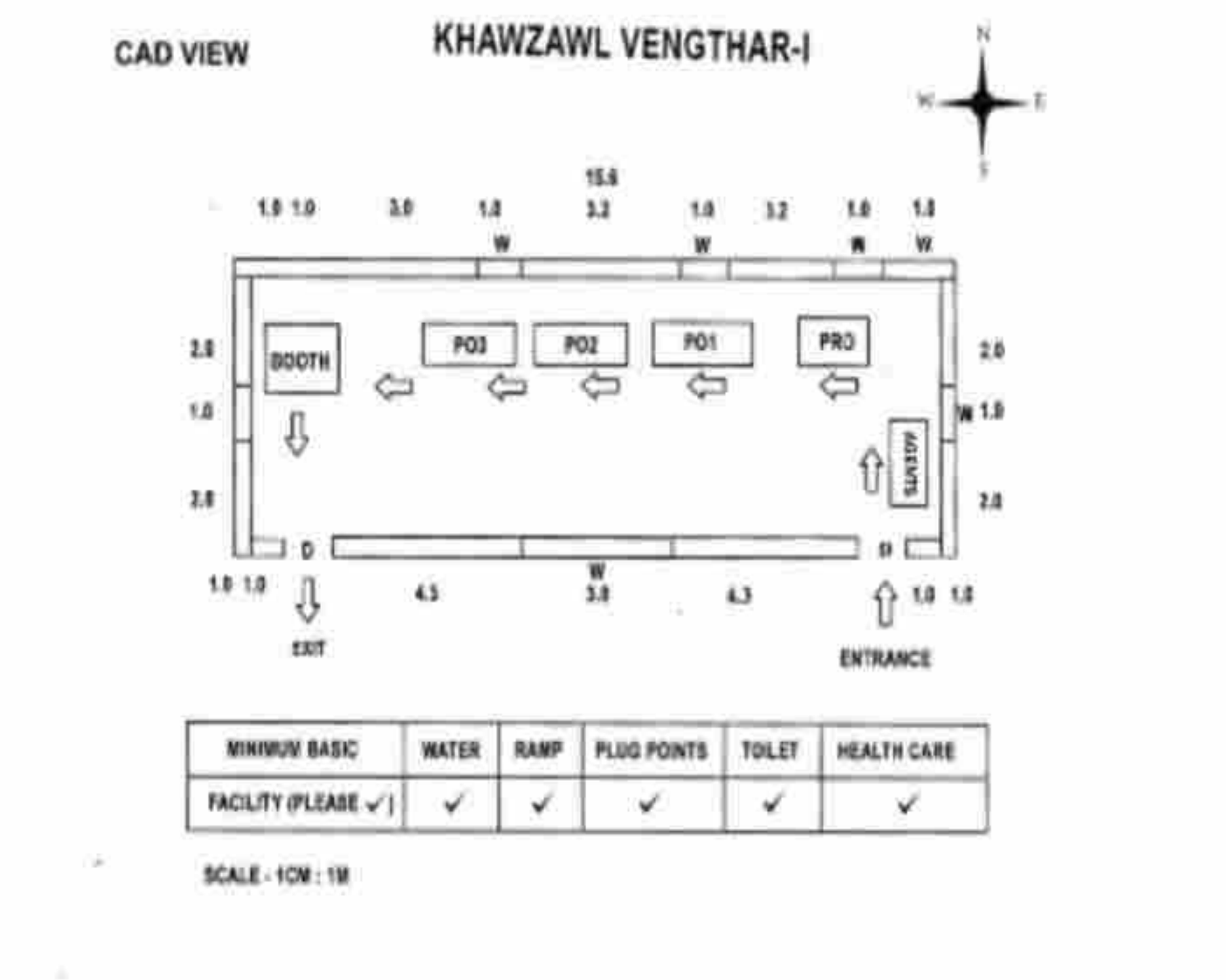
Cad View
