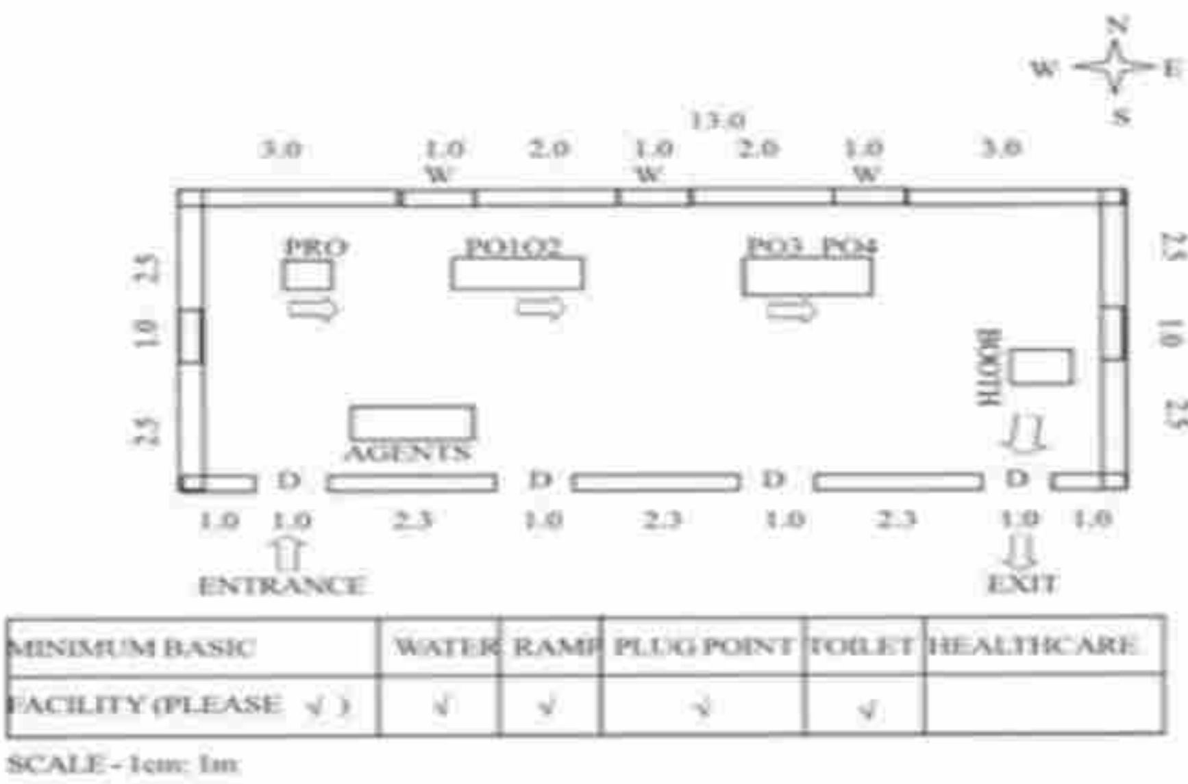
Cad View
